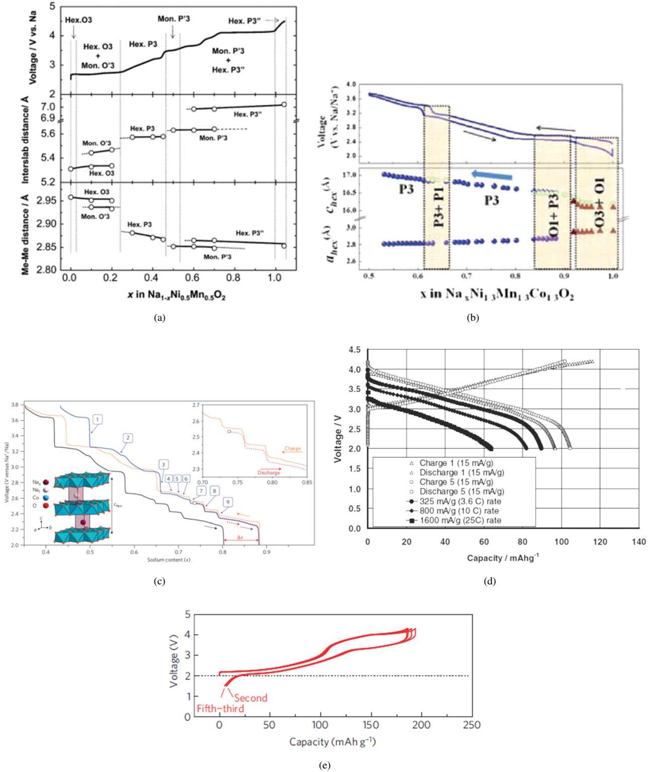
Fig. 3. The electrochemical voltage profiles of various layered oxide compounds: (a) \text{O3-NaNi}_{0.5}\text{Mn}_{0.5}\text{O}_2 , 12 (b) \text{O3-Na}[\text{Ni}_{1/3}\text{Mn}_{1/3}\text{Co}_{1/3}]\text{O}_2 , 15 (c) \text{P2-Na}_x\text{CoO}_2 , 16 (d) \text{P2-Na}_{1.0}\text{Li}_{0.2}\text{Ni}_{0.25}\text{Mn}_{0.75}\text{O}_2 , 21 (e) \text{P2-Na}_{2/3}[\text{Fe}_{1/2}\text{Mn}_{1/2}]\text{O}_2 . 22
