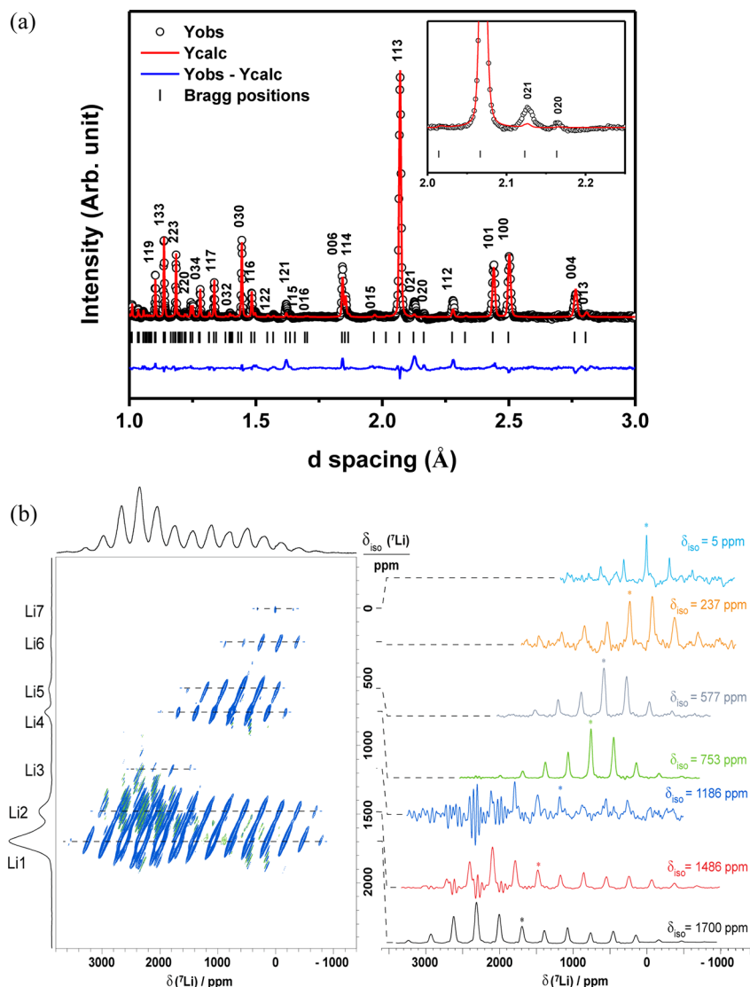
Figure 2. (a) Neutron diffraction patterns, including an extended view of the superlattice region (inset), and (b) the ^7\text{Li} aMAT NMR spectrum of as-synthesized \text{P2-Na}_{0.80}[\text{Li}_{0.12}\text{Ni}_{0.22}\text{Mn}_{0.66}]\text{O}_2 recorded at 500 MHz. In (b), the 1D double adiabatic spin echo (DASE) spectrum and the F1 sum spectrum are projected at the top and on the left-hand side of the 2D spectrum, respectively. Slices taken in the F2 dimension, centered about the ^7\text{Li} isotropic shifts, are shown on the right-hand side.
