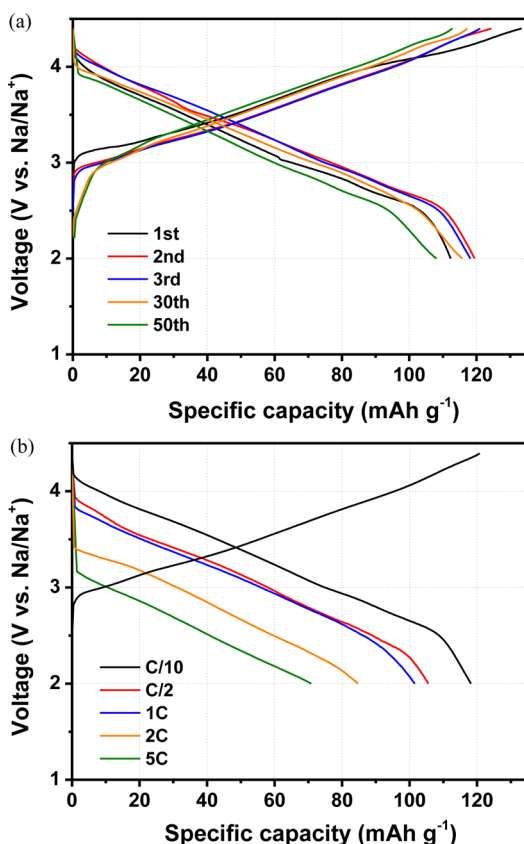
Figure 1. (a) Electrochemical profiles of \text{Na}_{0.8}[\text{Li}_{0.12}\text{Ni}_{0.22}\text{Mn}_{0.66}]\text{O}_2 during the 1st, 2nd, 3rd, 30th, and 50th cycles, and (b) its rate capability at different current densities from C/10 to 5C (calculated on the basis of a theoretical capacity of 118 \text{ mAh g}^{-1} ).
