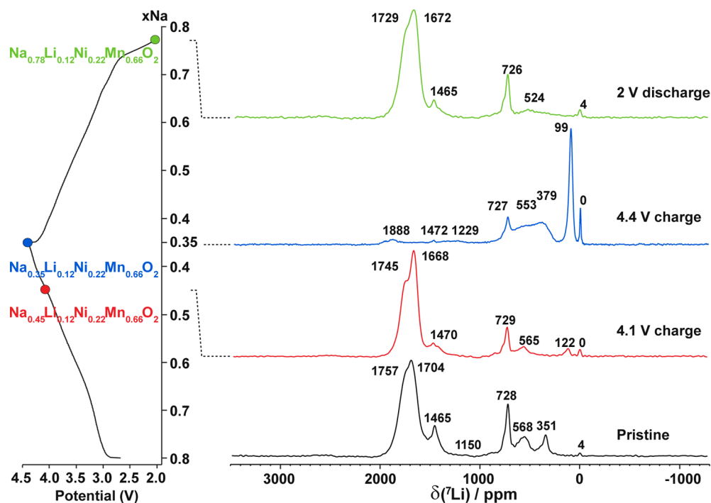
Figure 4. Isotropic slices of ^7\text{Li} pj-MATPASS NMR spectra acquired at 200 MHz on as-synthesized \text{P2-Na}_{0.8}[\text{Li}_{0.12}\text{Ni}_{0.22}\text{Mn}_{0.66}]\text{O}_2 and at three different stages along the first electrochemical cycle. pj-MATPASS experiments were performed using a train of five nonselective \pi/2 pulses. The spectra have not been scaled to represent the total Li content in the sample at each stage of the cycle.
