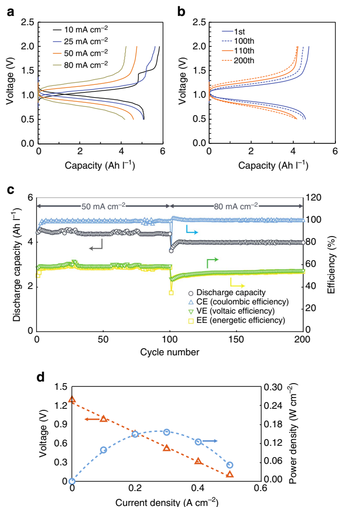
Figure 6 | Electrochemical performance of an FMN/Fe RFB at a high concentration. 0.4 M K 4 [Fe(CN) 6 ] in 1 M KOH aqueous positive electrolyte and 0.24 M FMN-Na and 1 M NA in 1 M KOH aqueous negative electrolyte were used. (a) Charge-discharge profiles at 10, 25, 50 and 80 mA cm -2 . (b) Charge-discharge curves at 1 st and 100 th cycles at 50 mA cm -2 , and 110 th and 200 th cycles at 80 mA cm -2 . (c) Cycling discharge capacities and efficiencies. (d) Voltage- and power-density dependencies on discharge current density.
