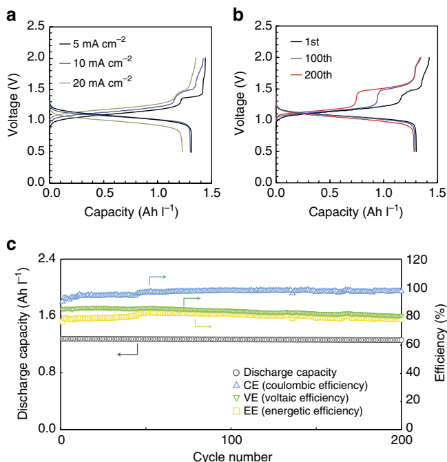
Figure 5 | Electrochemistry of an FMN/Fe RFB at a low concentration. 0.1 M K 4 [Fe(CN) 6 ] in 1 M KOH aqueous positive electrolyte and 0.06 M FMN-Na in 1 M KOH aqueous negative electrolyte were used. (a) Charge-discharge profiles at a current density of 5, 10 and 20 mA cm -2 . (b) Charge-discharge profiles at 1st, 100th, and 200th cycles at 10 mA cm -2 . (c) Cycling discharge capacity and efficiencies of an RFB at a current density of 10 mA cm -2 .
