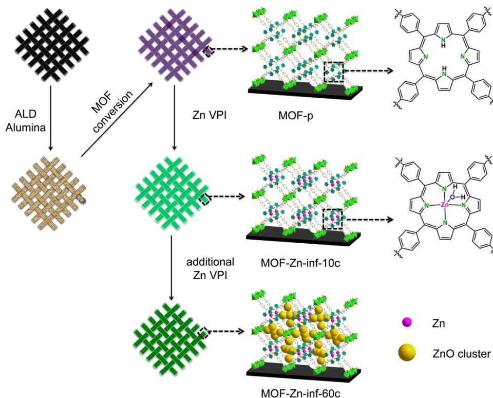
Figure 1. Schematic illustration of the MOF template and vapor phase infiltration. First, 10 nm of Al 2 O 3 was deposited onto the carbon fiber electrode by ALD. Then, the deposited Al 2 O 3 was reacted with TCPP to form MOF-p. Afterwards, the diethyl zinc and H 2 O precursors were alternately introduced to the porous MOF structure to coordinate with the porphyrin ( \leq 10 cycles). Finally, additional VPI cycles ( > 10 cycles) were run to form ZnO clusters inside the MOF pores and induce internal strain. Pink indicates Zn atoms occupying central MOF positions and yellow indicates ZnO clusters inside the MOF pores.
