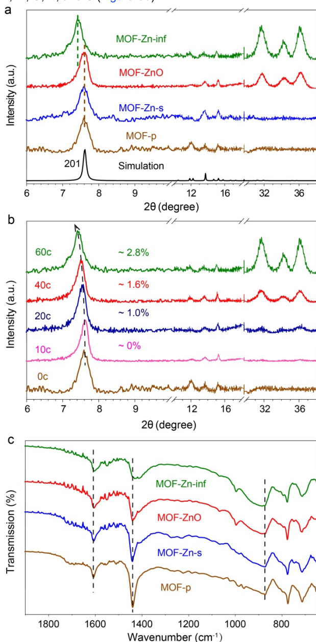
Figure 3. XRD and FTIR characterizations. a , XRD of MOF samples on carbon fiber electrodes. b , XRD of VPI samples with various infiltration cycles. c , FTIR of MOF samples on Si substrates.
