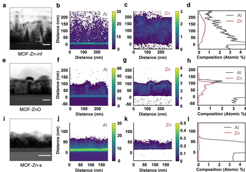
Figure 2. Structural characterization and chemical profiling. a, e, i, STEM images of MOF-Zn-inf, MOF-ZnO and MOF-Zn-s, respectively. Scale bar: 50 nm. b-c, f-g, j-k, EDS mappings of Al and Zn. d, h, l, STEM EDS line profiling coupled with spectral components, atomic percentages, and elemental depth.
