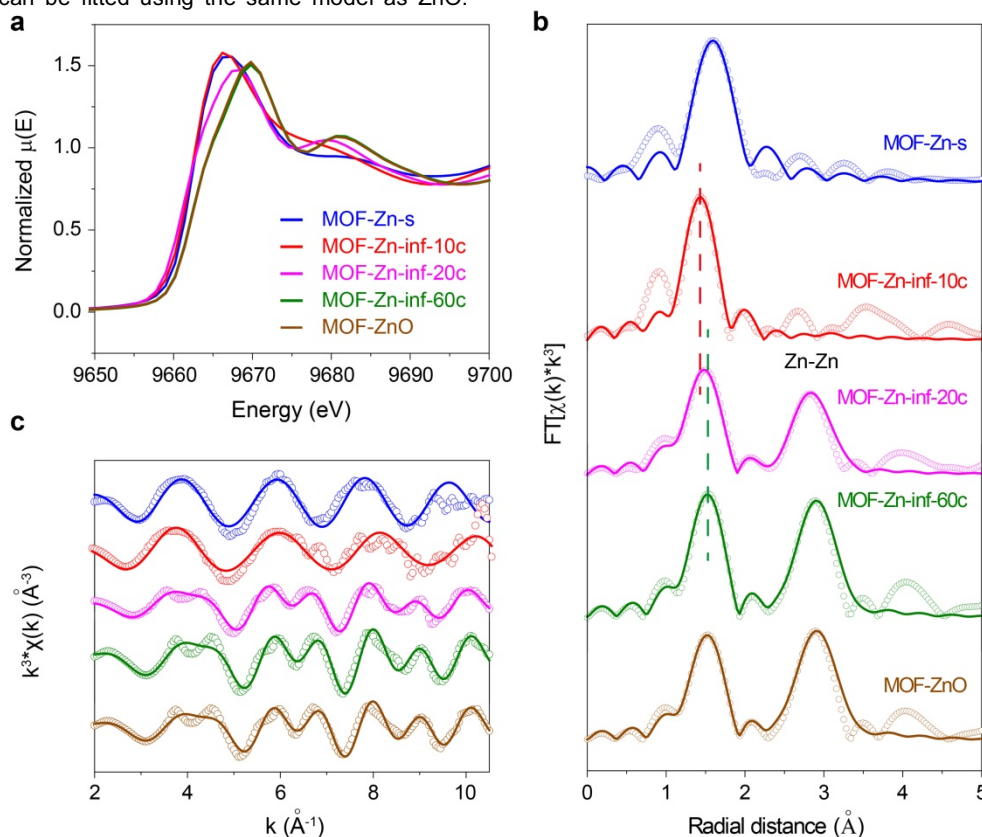
Figure 4. X-ray absorption analysis. a , Normalized Zn K-edge XANES spectra. b , Corresponding EXAFS spectra (open dots) and their fitting results (solid lines) in R-space. Dashed lines indicate the peak position of Zn-ligand first shell for MOF-Zn-inf-10c and MOF-Zn-inf-60c. c , Corresponding EXAFS spectra (open dots) and their fitting results (solid lines) in K-space.
