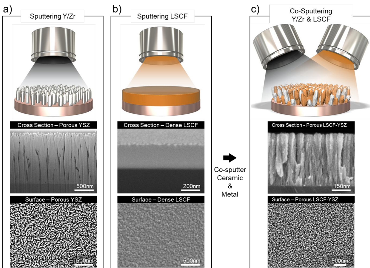
Figure 1. Schematic of sputtering metal, ceramic and co-sputtering of metal and ceramic. (a) Sputtering of a Y/Zr metal alloy target and the corresponding porous YSZ cross-sectional and
